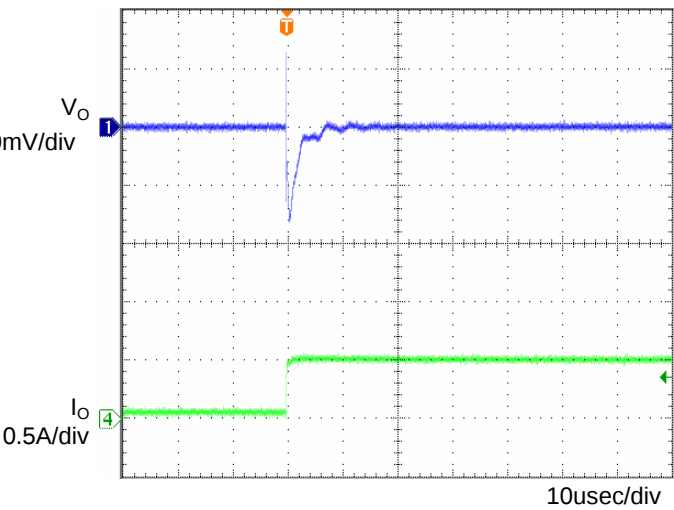
Fig.4 Transient Response (0→0.5A) Co=1 \mu F, Ta=25°C
