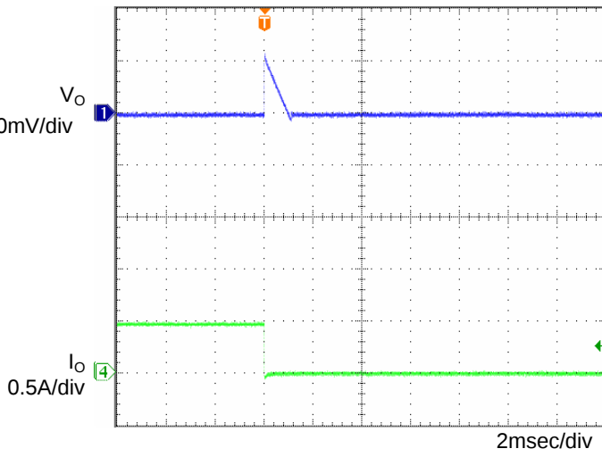
Fig.6 Transient Response (0.5→0A) Co=1 \mu F, Ta=-40°C
