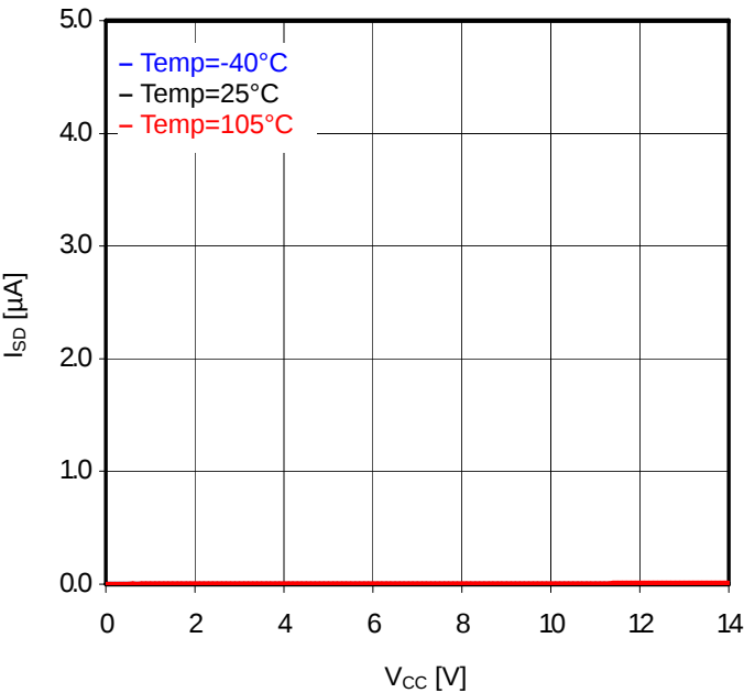
Fig. 26 V_{CC}-I_{SD} ( V_{EN}=0V )
