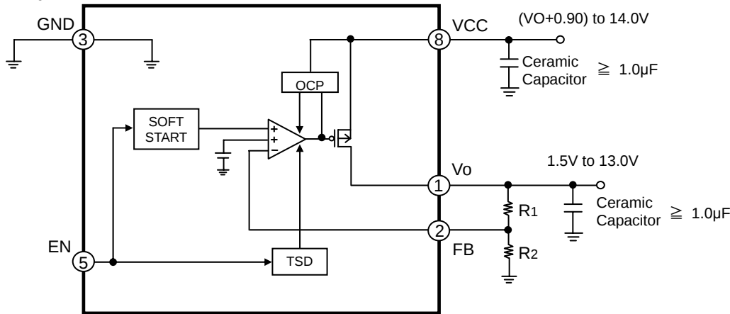
Fig.1 Block Diagram
