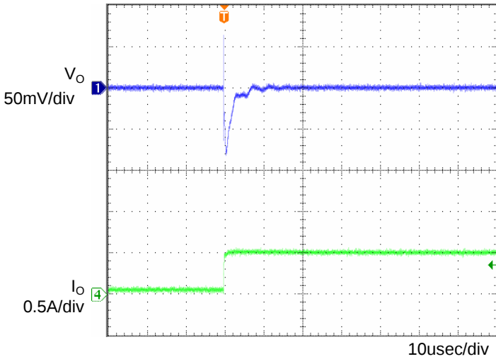
Fig.4 Transient Response (0 \rightarrow 0.5A) Co=1 \mu F, Ta=25°C
