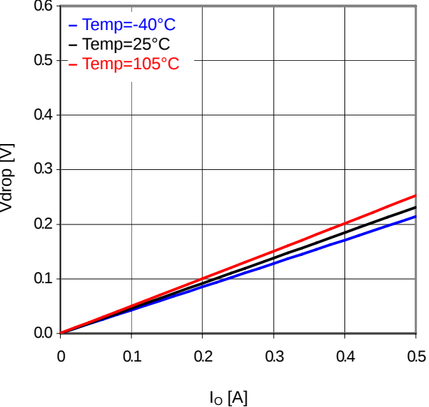
Fig. 38 Minimum dropout Voltage 5 (V CC =12.0V)
