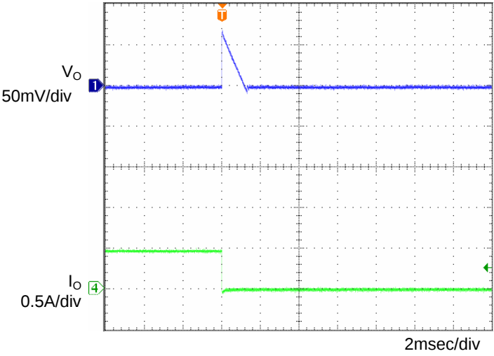
Fig.8 Transient Response (0.5→0A) Co=1μF, Ta=105°C
