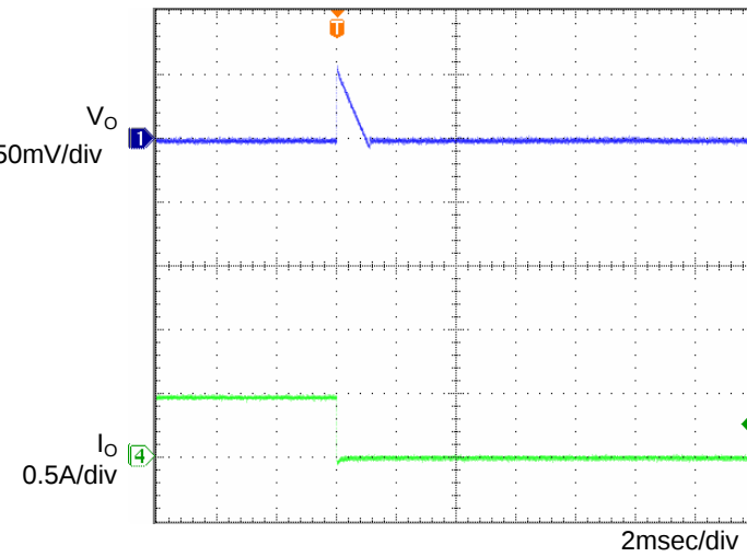
Fig.6 Transient Response (0.5→0A) Co=1 \mu F, Ta=-40°C
