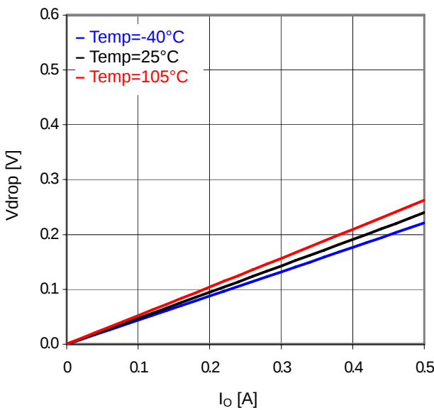
Fig. 37 Minimum dropout Voltage 4 (V CC =10.0V)
