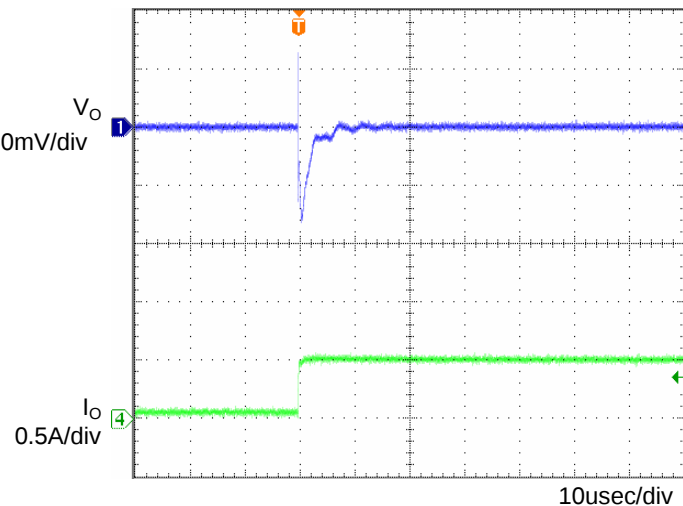
Fig.4 Transient Response (0→0.5A) Co=1 \mu F, Ta=25°C
