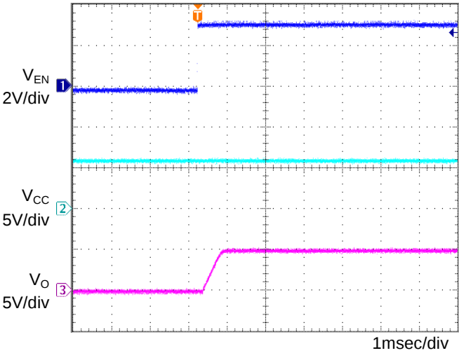
Fig.17 Input sequence 2 \text{Co}=1\mu\text{F} , T_a=105^{\circ}\text{C}
