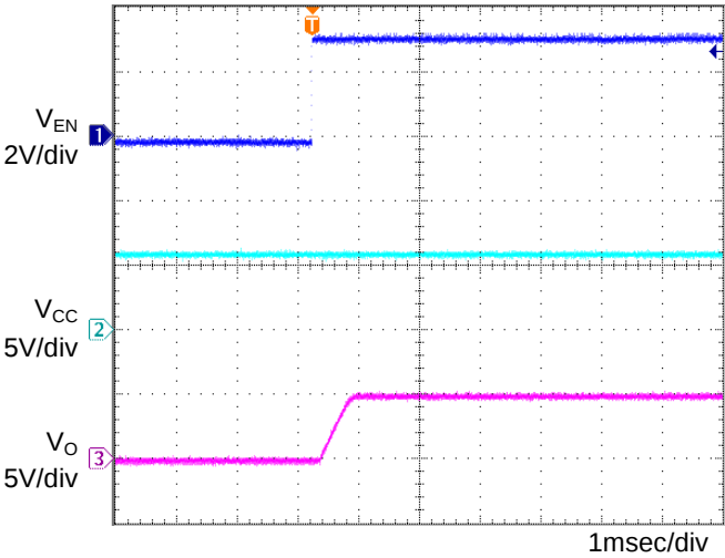
Fig.15 Input sequence 2 \text{Co}=1\mu\text{F} , T_a=-40^{\circ}\text{C}
