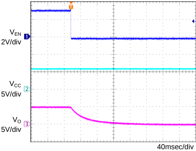
Fig.18 OFF sequence 2 \text{Co}=1\mu\text{F} , T_a=-40^{\circ}\text{C}
