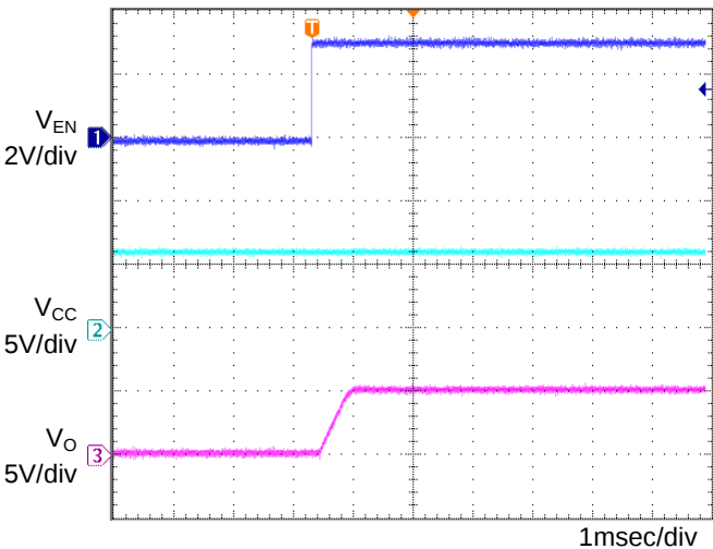
Fig.16 Input sequence 2 \text{Co}=1\mu\text{F} , T_a=25^{\circ}\text{C}
