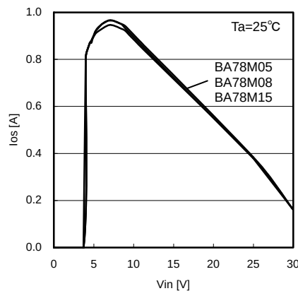
Fig.8 Short - Circuit Output Current
