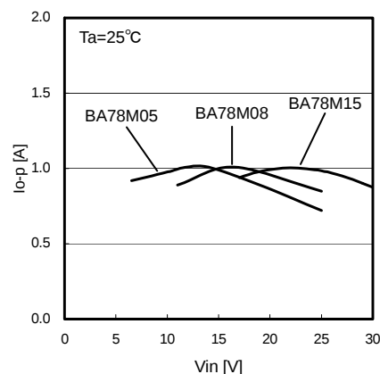
Fig.6 Peak Output Current
