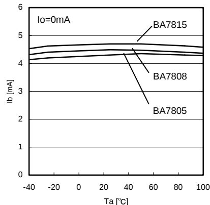
Fig.23 T_a - I_b
