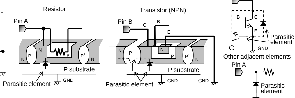
Fig.28 Simplified structure of monoristic IC
