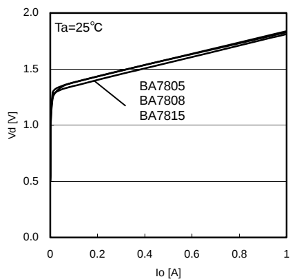
Fig.19 Dropout Voltage
