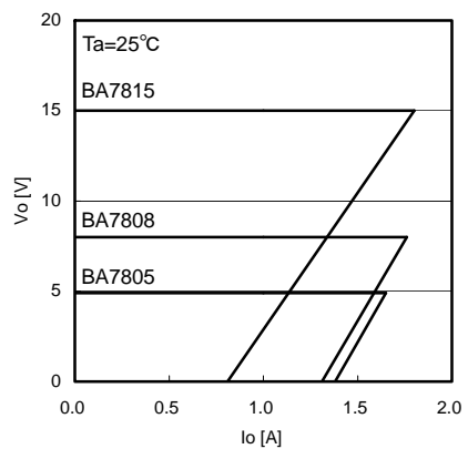
Fig.17 Load Regulation
