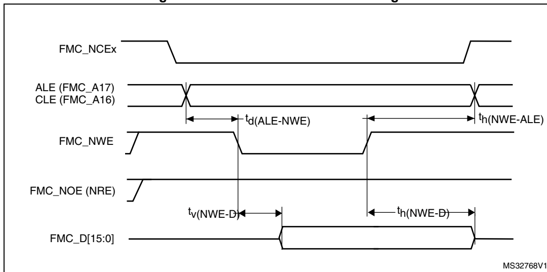
Figure 35. NAND controller write timings
