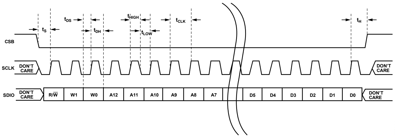
Figure 58. Serial Port Interface Timing Diagram
