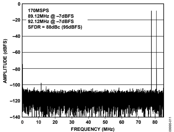
Figure 12. AD9642-170 Two-Tone FFT with f_{IN1} = 89.12 MHz, f_{IN2} = 92.12 MHz
