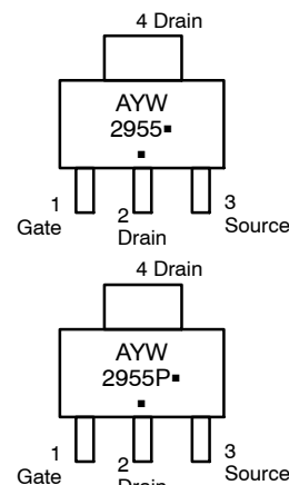
SOT–223 CASE 318E STYLE 3
