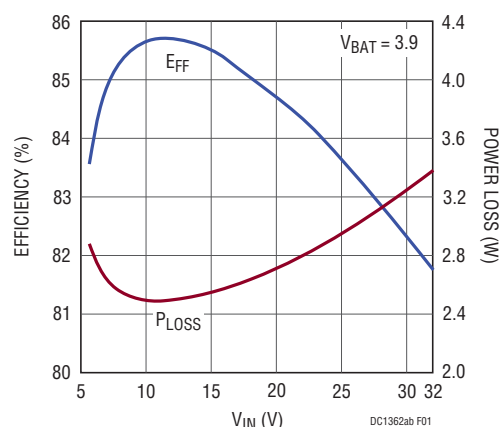
Figure 1. Efficiency and Power Loss vs V_{\text{IN}}
