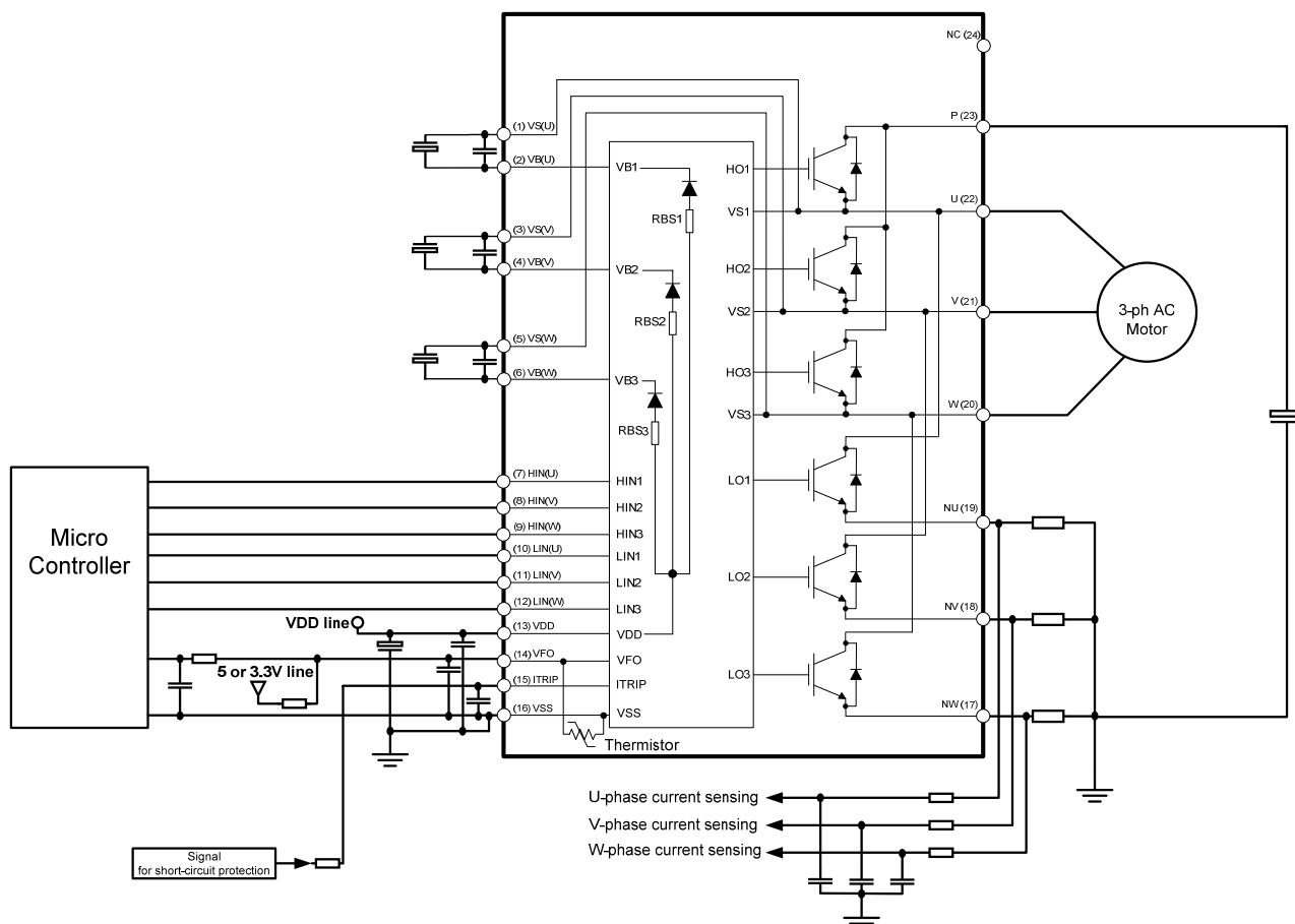
Figure 9: Application circuit
