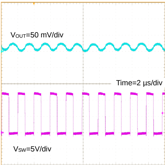
Figure 29. V_{OUT} Ripple ( V_{IN} =12 V, V_{OUT} =5 V, I_{OUT} =1 A, C_{OUT} =10 \mu Fx3)
