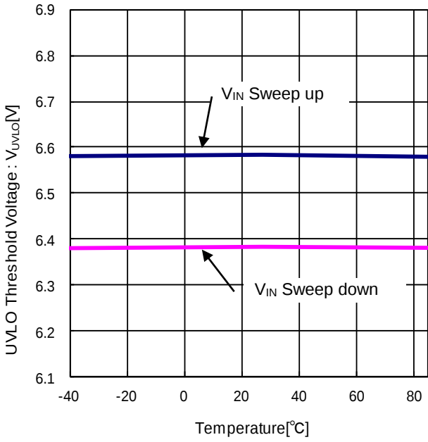
Figure 13. UVLO Threshold Voltage vs Temperature
