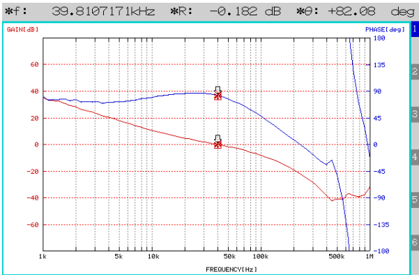
Figure 35. Loop Response ( V_{IN}=12\text{ V} , V_{OUT}=3.3\text{ V} , I_{OUT}=1\text{ A} , C_{OUT}=\text{Ceramic}10\text{ }\mu\text{F}\times 3 )
