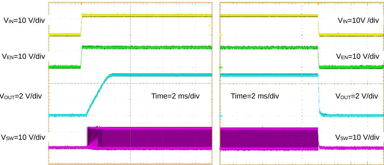
Figure 22. Start-up Waveform ( V_{IN}=V_{EN} ) I_{OUT}=1.0 A
