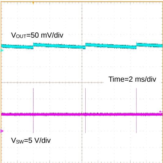
Figure 26. V_{OUT} Ripple ( V_{IN} =12 V, V_{OUT} = 5 V, I_{OUT} =0 A, C_{OUT} =10 \mu Fx3)
