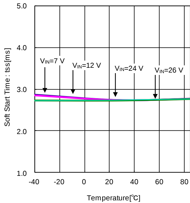
Figure 17. Soft Start Time vs Temperature
