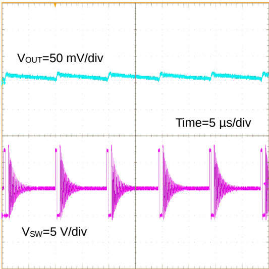
Figure 27. V_{OUT} Ripple ( V_{IN} =12 V, V_{OUT} =5 V, I_{OUT} =10 mA, C_{OUT} =10 \mu Fx3)
