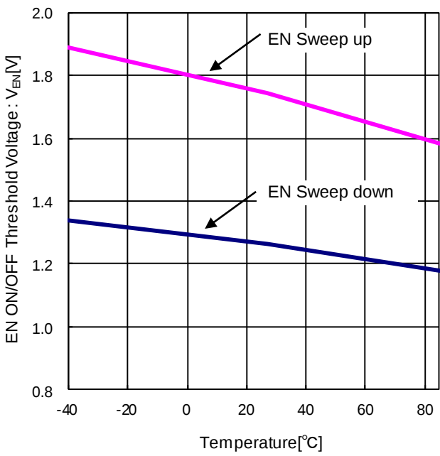
Figure 15. EN ON/OFF Threshold Voltage vs Temperature
