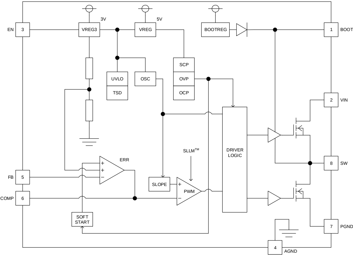
Figure 3. Block Diagram
