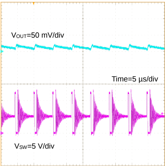
Figure 28. V_{OUT} Ripple ( V_{IN} =12 V, V_{OUT} =5 V, I_{OUT} =20 mA, C_{OUT} =10 \mu Fx3)
