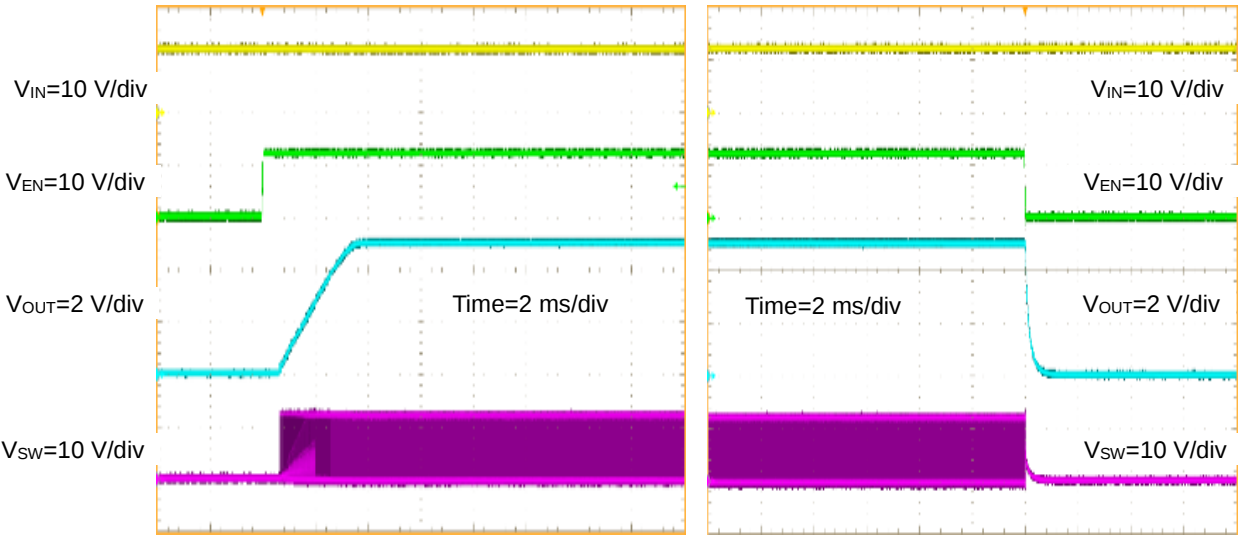
Figure 24. Start-up Waveform ( V_{EN}=0 V to 5 V) I_{OUT}=1.0 A
