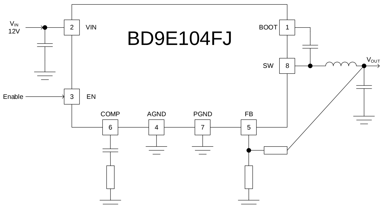
Figure 1. Application Circuit
