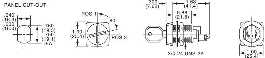
PANEL CUT-OUT
