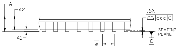
Figure 17. 16-Pin Small Outline Integrated Circuit (SOIC) Package
