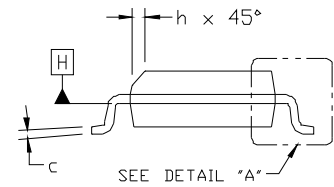
Figure 17. 16-Pin Small Outline Integrated Circuit (SOIC) Package
