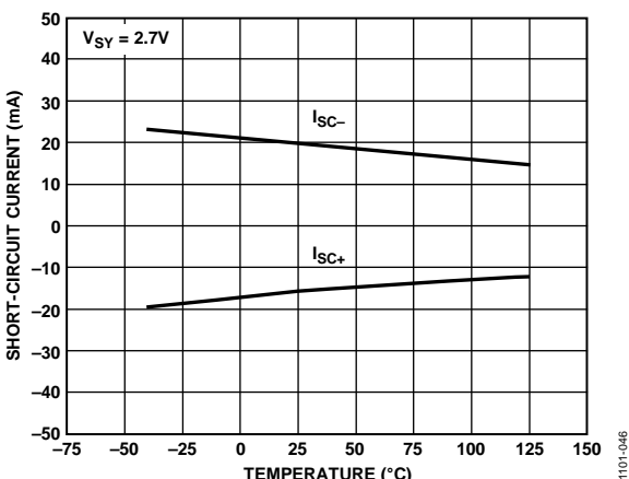
Figure 46. Output Short-Circuit Current vs. Temperature
