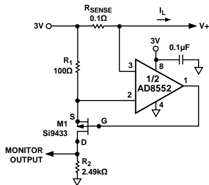
Figure 69. A High-Side Load Current Monitor
