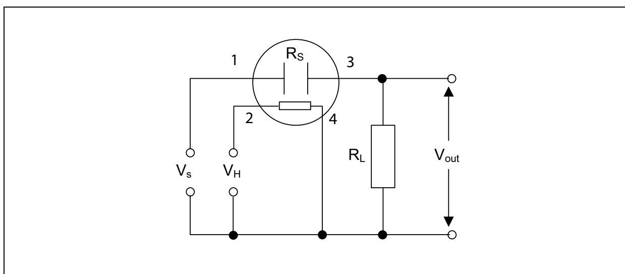
Figure 8: A Basic Measurement Circuit for the Sensor Resistance
