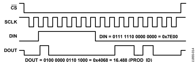
Figure 17. SPI Read Example, Second 16-Bit Sequence
