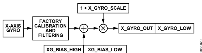
Figure 22. User Calibration Signal Path, Gyroscopes
