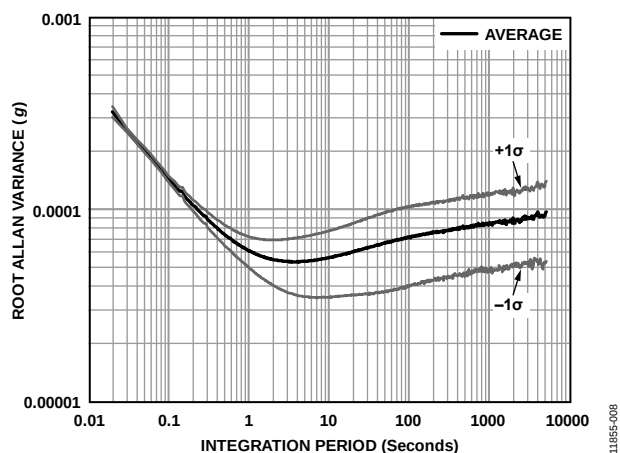
Figure 8. Accelerometer Allan Variance, 25°C
