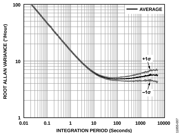
Figure 7. Gyroscope Allan Variance, 25°C
