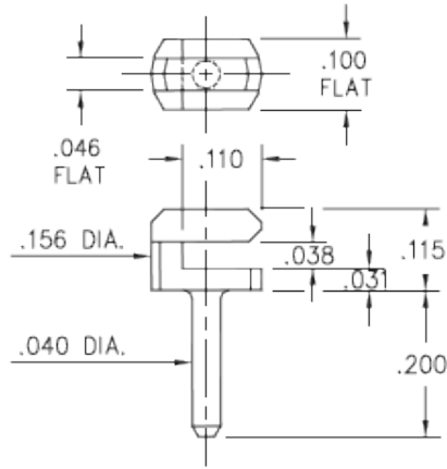
7310-0-01-XX-00-00-08-0 Board edge press-fit
