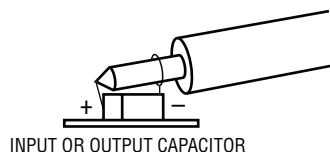
Figure 2. Proper Scope Probe Technique for Measuring Input or Output Ripple
