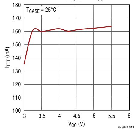
Total Current ( I_{\text{TOT}} ) vs V_{CC}
