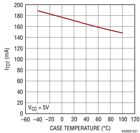
Total Current ( I_{\text{TOT}} ) vs Case Temperature
