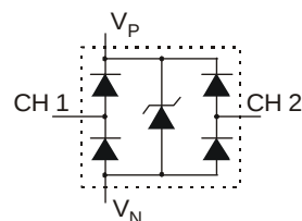
Device Schematic
