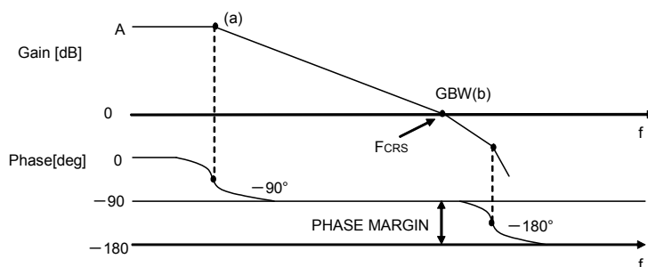
Figure 52. Bode Plot
