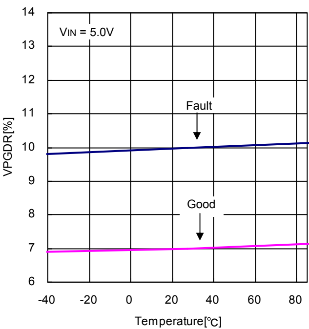
Figure 17. PGD Rising Voltage vs Temperature
