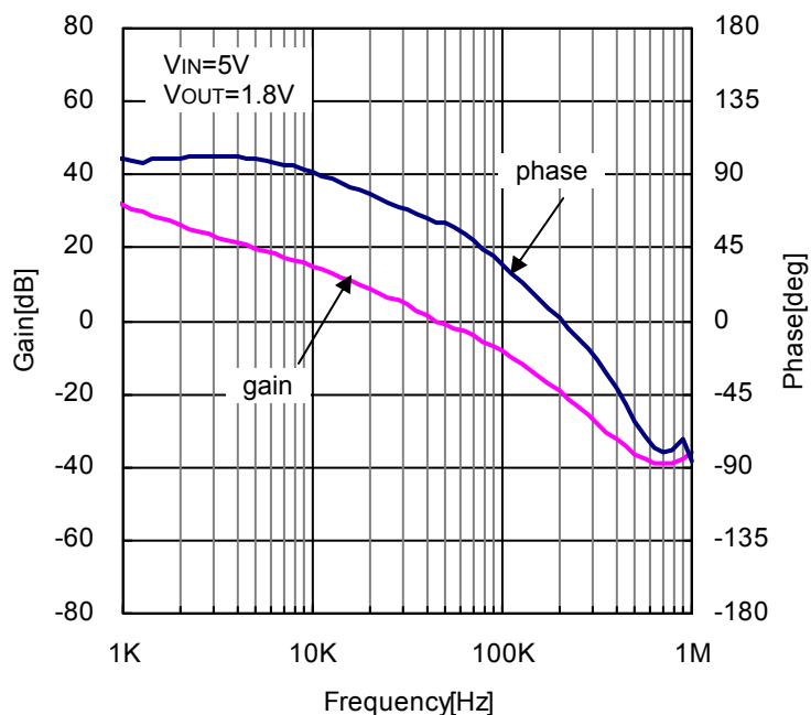
Figure 25. Closed Loop Response ( V_{IN}=5V , V_{OUT}=1.8V , L=2.2\mu H , C_{OUT}=\text{Ceramic } 44\mu F )
