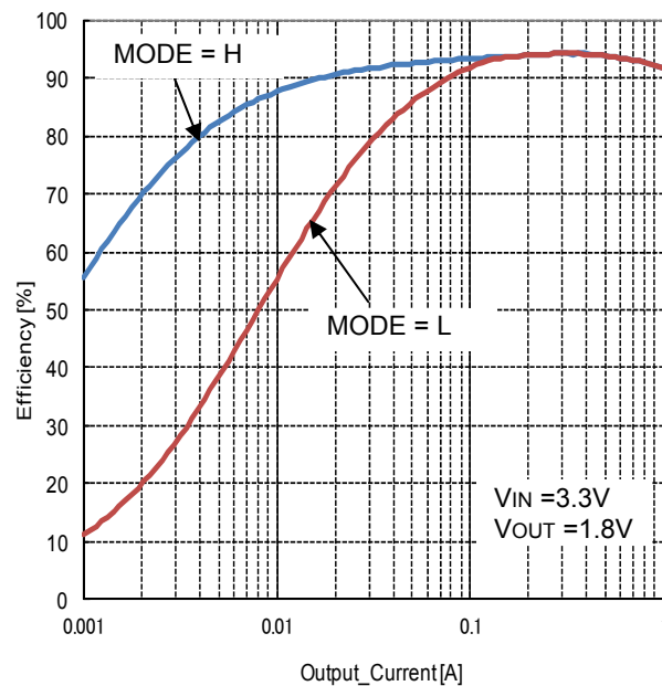
Figure 23. Efficiency vs Load Current ( V_{IN}=3.3V , V_{OUT}=1.8V , L=2.2\mu H )
