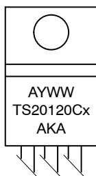
TO-220AB
