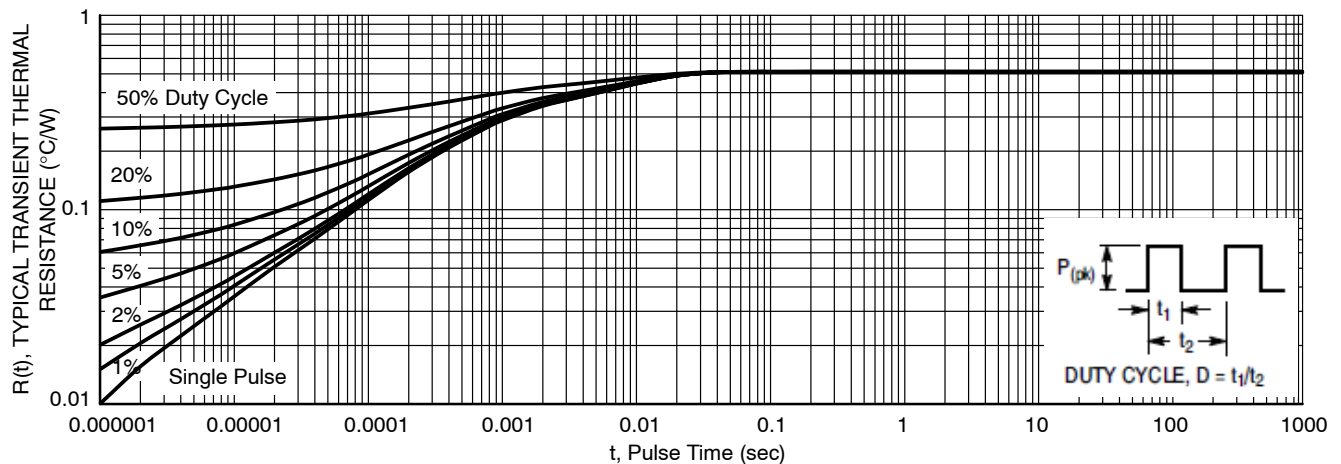
Figure 9. Typical Transient Thermal Response for NTSB20120CTG
