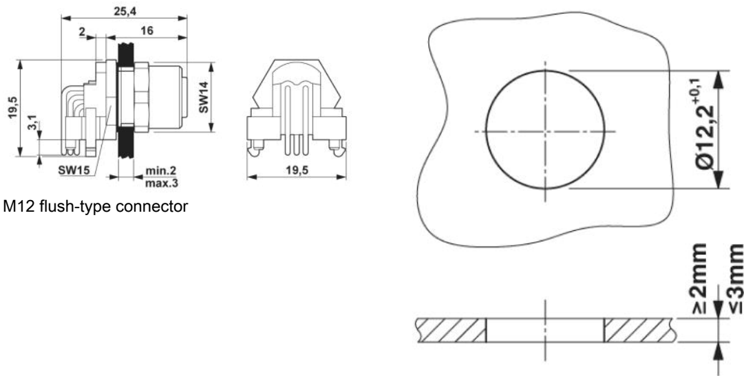
Panel cutout
