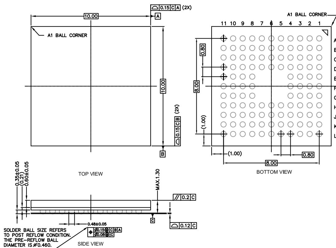
Figure 4.3. BGA112
