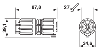
Dimensional drawing
