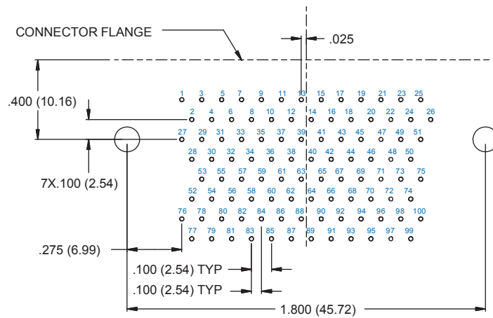
100 PIN
