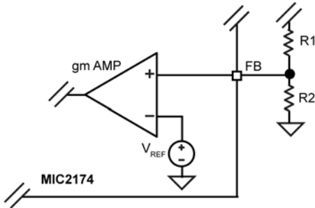
Figure 8. Voltage-Divider Configuration
