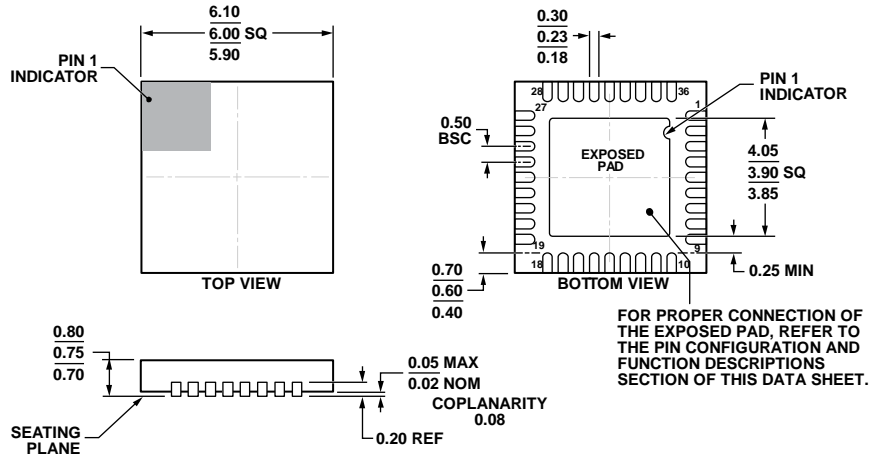
COMPLIANT TO JEDEC STANDARDS MO-220-WJJD. Figure 47. 36-Lead Lead Frame Chip Scale Package [LFCSP_WQ] 6 mm x 6 mm Body, Very Very Thin Quad (CP-36-3) Dimensions shown in millimeters
