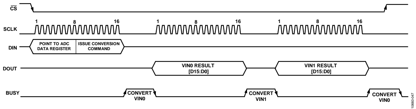
Figure 41. ADC Conversion Command (ADC Sequencer Used)
