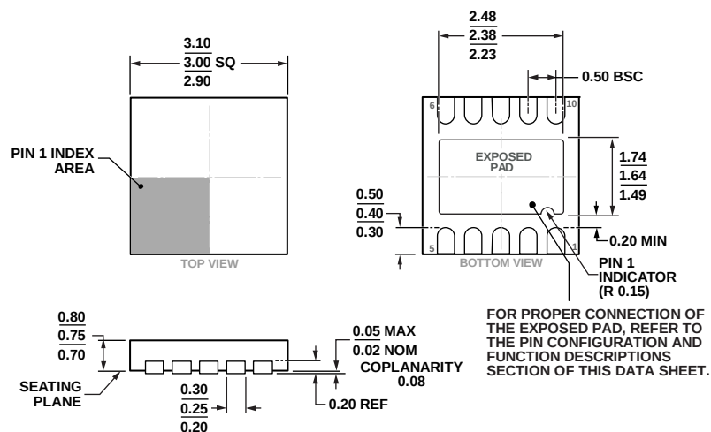
Figure 36. 10-Lead Lead Frame Chip Scale Package [LFCSP_WD]
