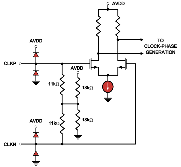
FIGURE 49. CLOCK INPUTS
