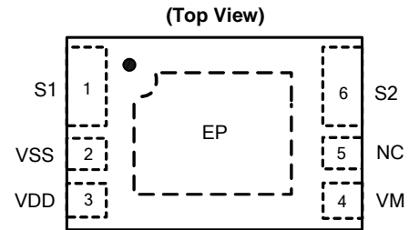
U-DFN2535-6 (Option 1)
