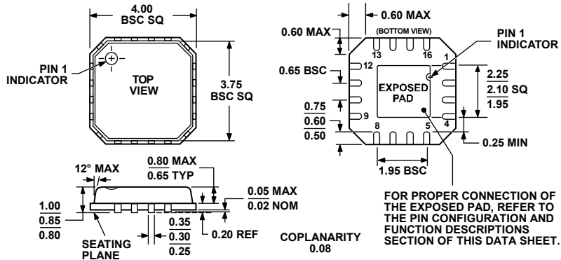
COMPLIANT TO JEDEC STANDARDS MO-220-VGGC Figure 43. 16-Lead Lead Frame Chip Scale Package [LF CSP_VQ] 4 mm x 4 mm Body, Very Thin Quad (CP-16-4) Dimensions shown in millimeters
