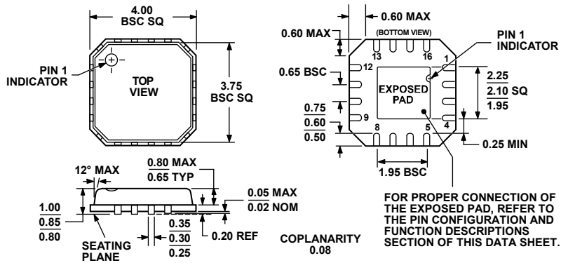
Figure 43. 16-Lead Lead Frame Chip Scale Package [LF CSP_VQ]
