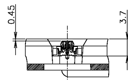
E-E (SCALE 2:1)
