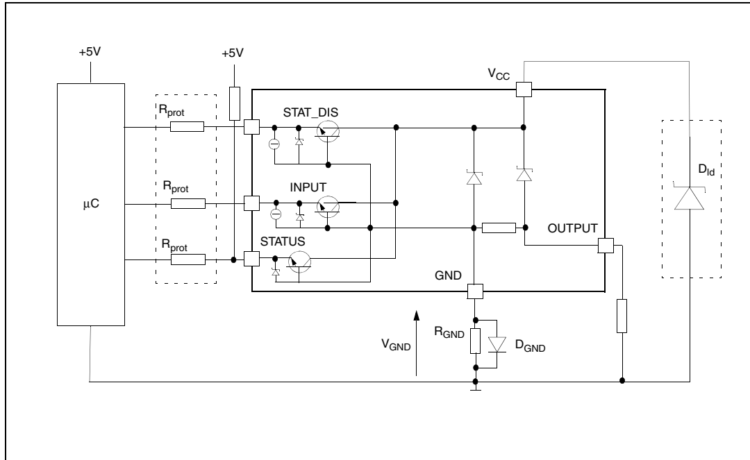
Figure 32. Application schematic
