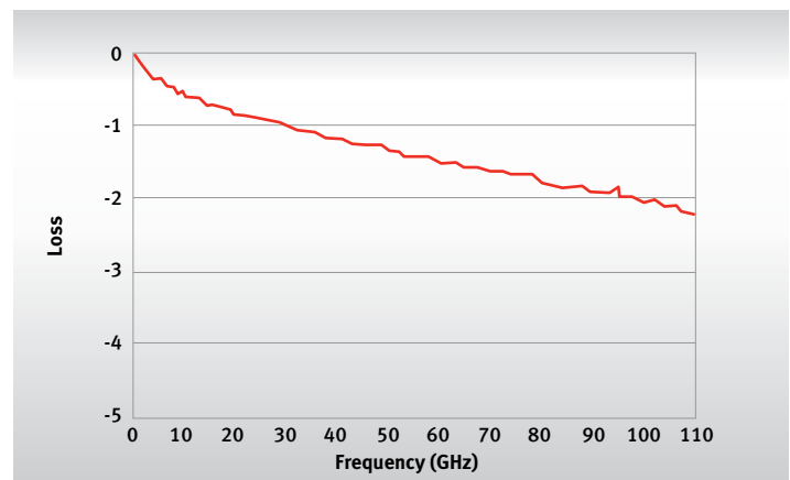
FIGURE 4: TYPICAL INSERTION LOSS 1
