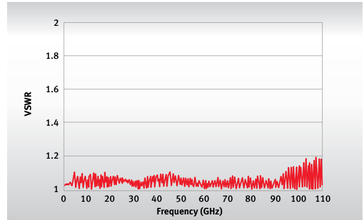
FIGURE 3: TYPICAL VSWR 1
