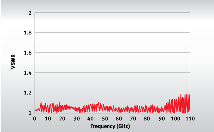
FIGURE 3: TYPICAL VSWR 1
