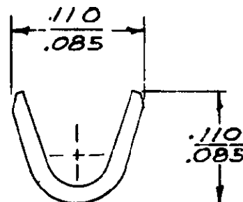
SECT. "A-A"
