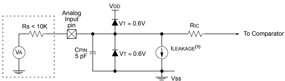
FIGURE 17-3: ANALOG INPUT MODEL
