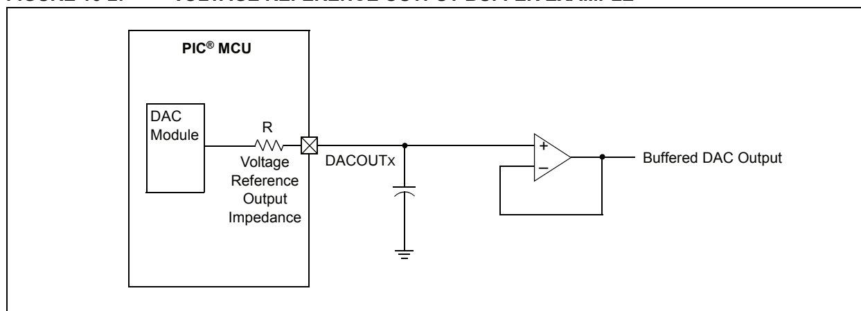
FIGURE 16-2: VOLTAGE REFERENCE OUTPUT BUFFER EXAMPLE
