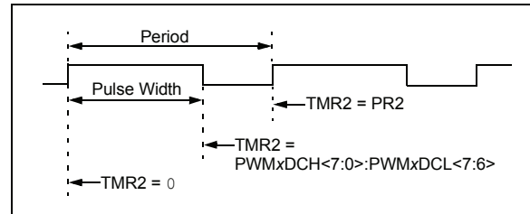
FIGURE 21-1: PWM OUTPUT
