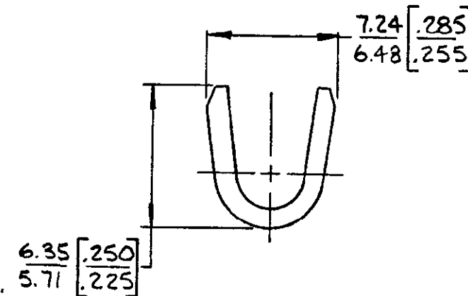
SECT B-B
