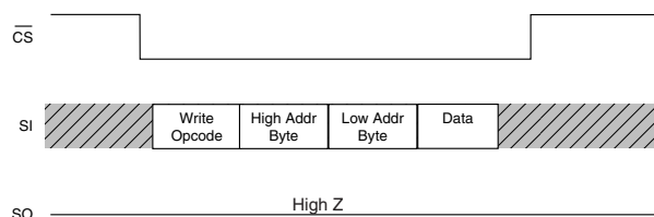
FIGURE 9. Byte Write
