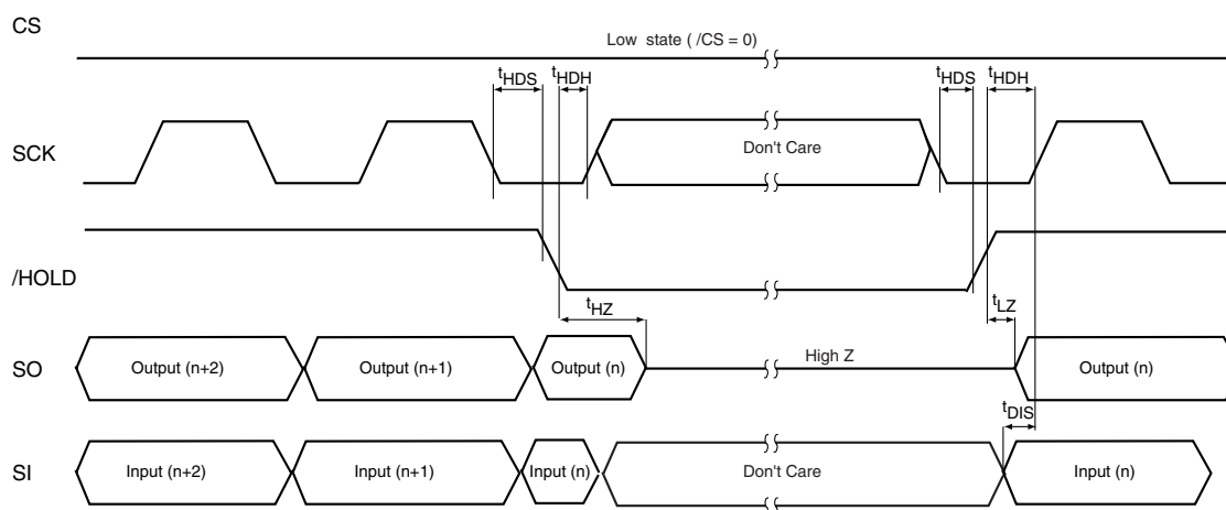
FIGURE 3. HOLD Timing
