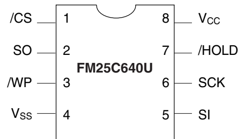
Dual-In-Line Package (N) and SO Package (M8)
