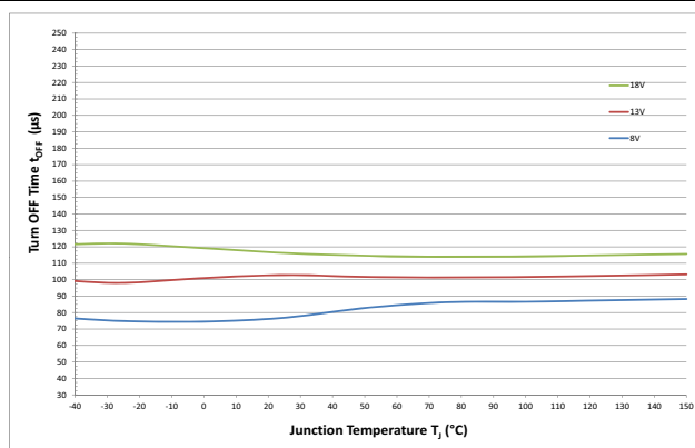
Figure 38 Turn OFF t_{OFF} = f(T_J; V_S) , R_L = 2 \Omega
