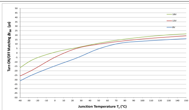
Figure 39 Turn ON / OFF matching \Delta t_{SW} = f(T_J; V_S) , R_L = 2 \Omega
